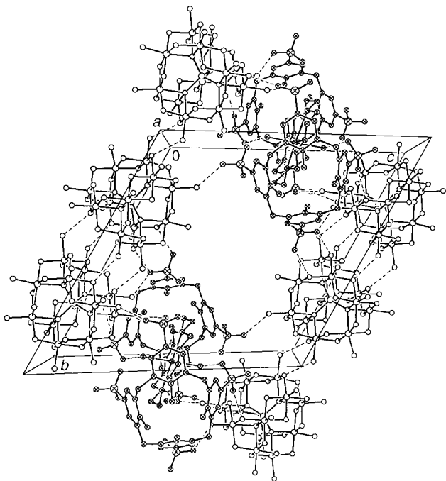
Fig. 3 Interplay of Keggin ions and superanions (shown cross-hatched) within [\text{Al}_{13}\text{O}_4(\text{OH})_{24}(\text{H}_2\text{O})_{12}][\text{Na}(18\text{-crown-6})(\text{H}_2\text{O})_2\text{L}_2\text{-(H}^+)_w]_{0.5}^{x-}[\text{L}(\text{H}^+)]_z^{z-} \cdot 29\text{H}_2\text{O} , 1 , x + z = 7 , viewed down the a axis. The Keggin ions [\text{Al}_{13}\text{O}_4(\text{OH})_{24}(\text{H}_2\text{O})_{12}]^{7+} run in infinite hydrogen bonded chains along the b direction with inter-Keggin \text{O} \cdots \text{O} separations ranging from 2.70 to 2.85 Å. Solvent water and the water-bearing calix[4]arene are not shown for clarity and occupy the apparent spaces within the cell.
